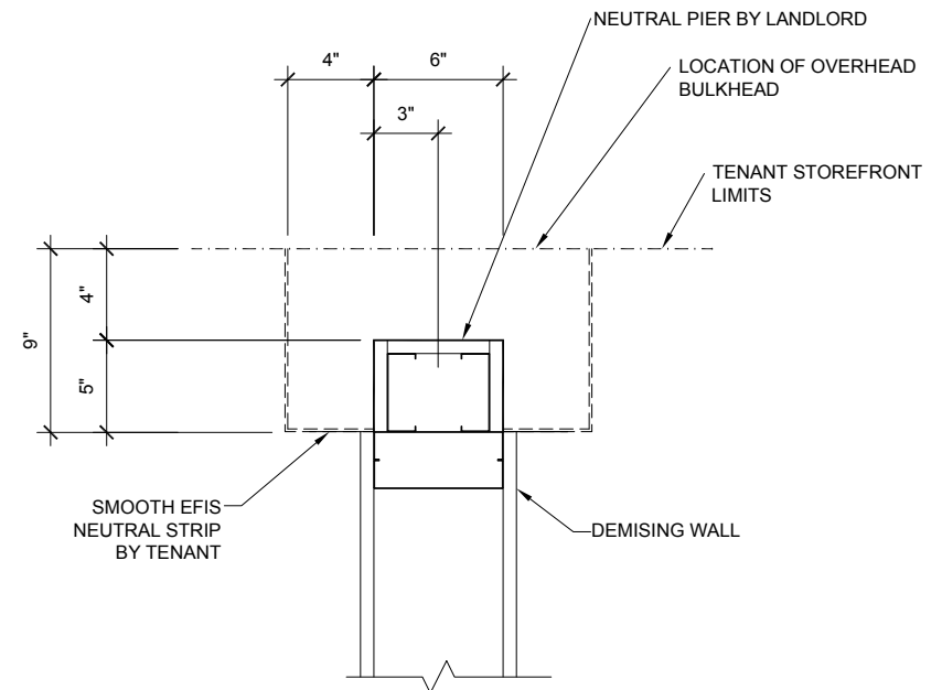
TYPICAL NEUTRAL PIER DETAIL
