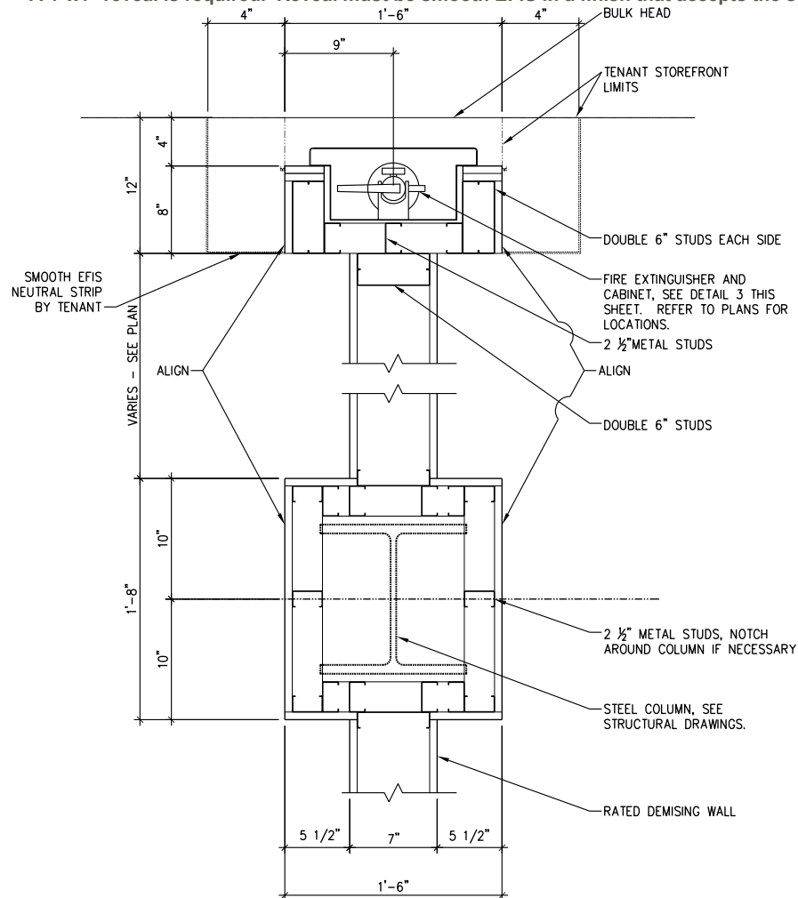
WITH FIRE EXTINGUISHER CABINET
